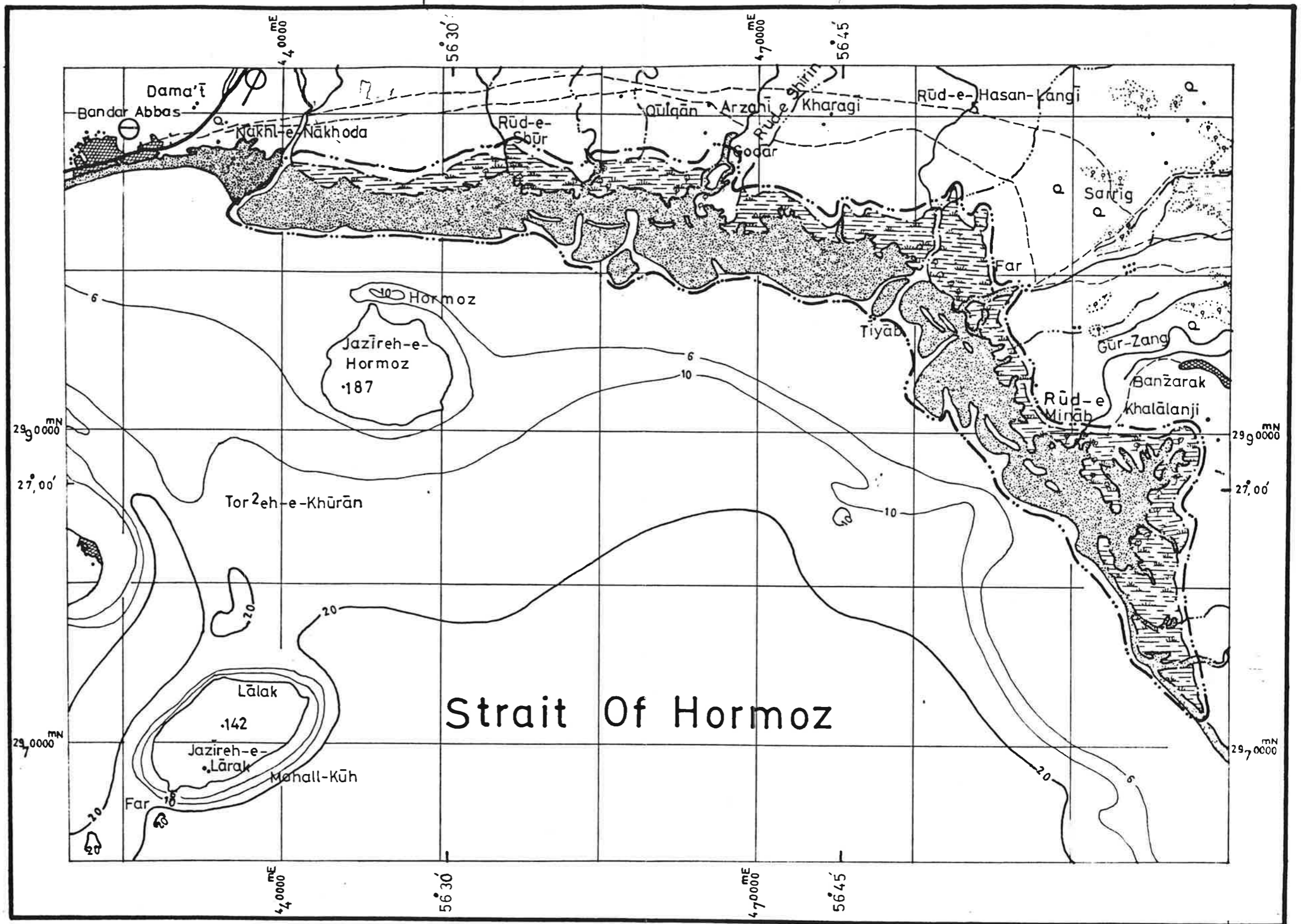
16 Deltas Of Rud-e-Shur, Rud-e-Shirin And Rud-e-Minab
