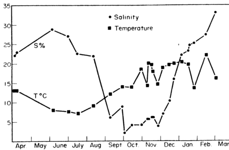
Figure 3.8: (a). Salinity and temperature in Orielton Lagoon April 1975-March 76. (Source: Buttermore 1977)
