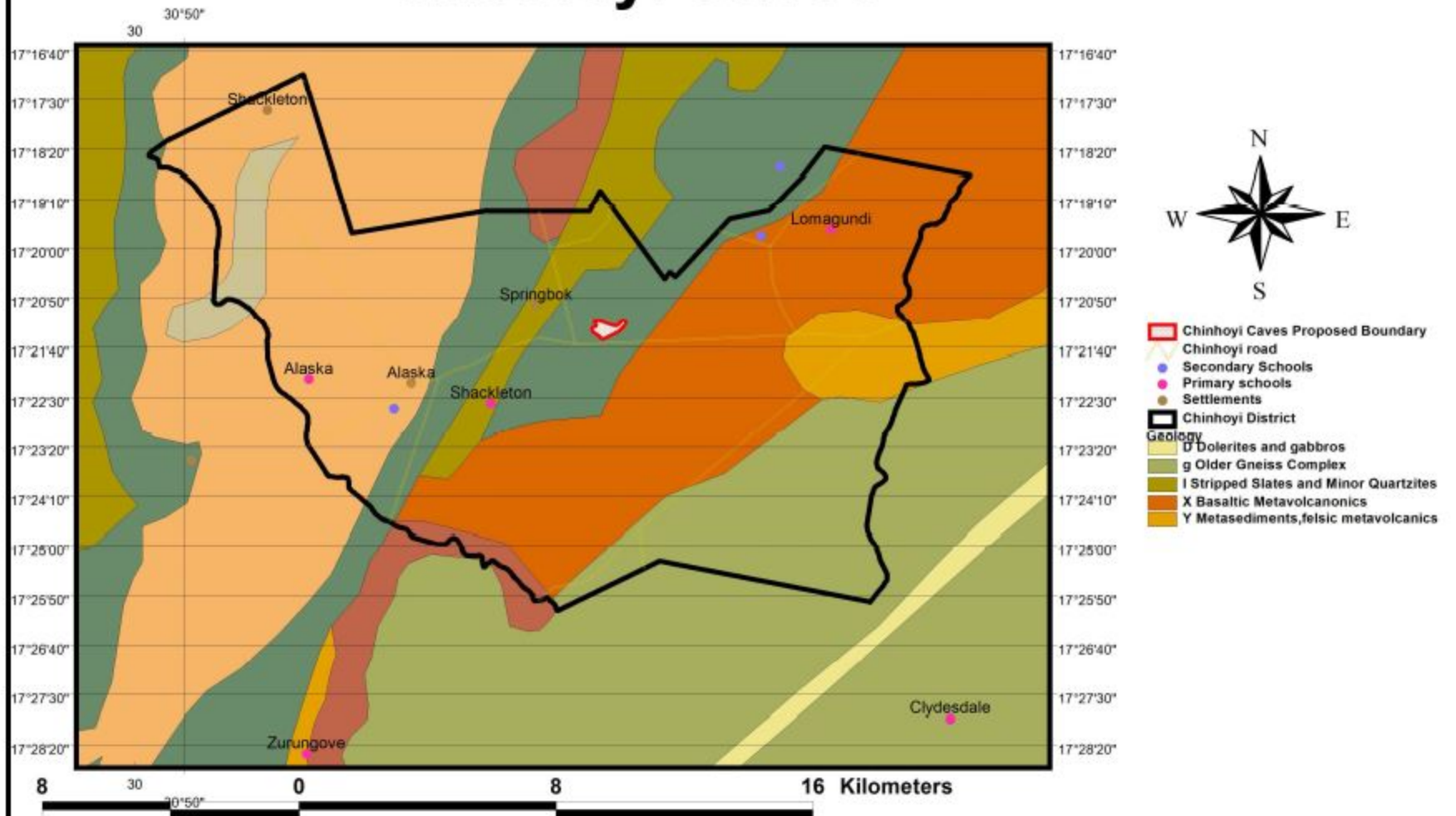
Geology Map of Chinhoyi Caves
